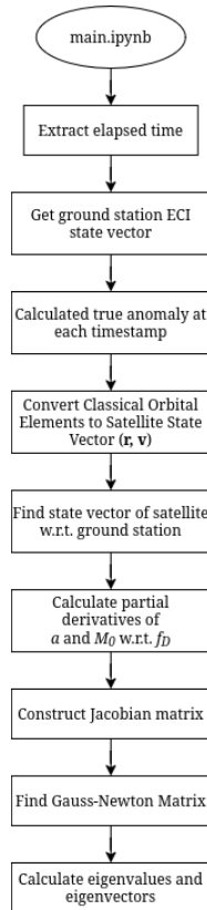
Figure 1: Block diagram of main code
